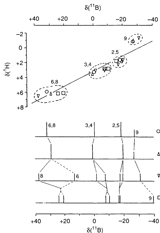
Fig. 1 Selected NMR data for compounds 1 (○), 2 (□), 3 (▽) and 5 (△). The bottom set of diagrams are stick representations of the chemical shifts and relative intensities in the 11 B spectra, with lines joining equivalent positions in the four compounds. Hatched lines join the P-substituted positions for compounds 2 and 3 . The top diagram plots δ( 1 H) versus δ( 11 B) for the {BH} units in the four compounds. The line drawn has slope δ( 11 B):δ( 1 H) 10:1, intercept +3.20 in δ( 1 H)
